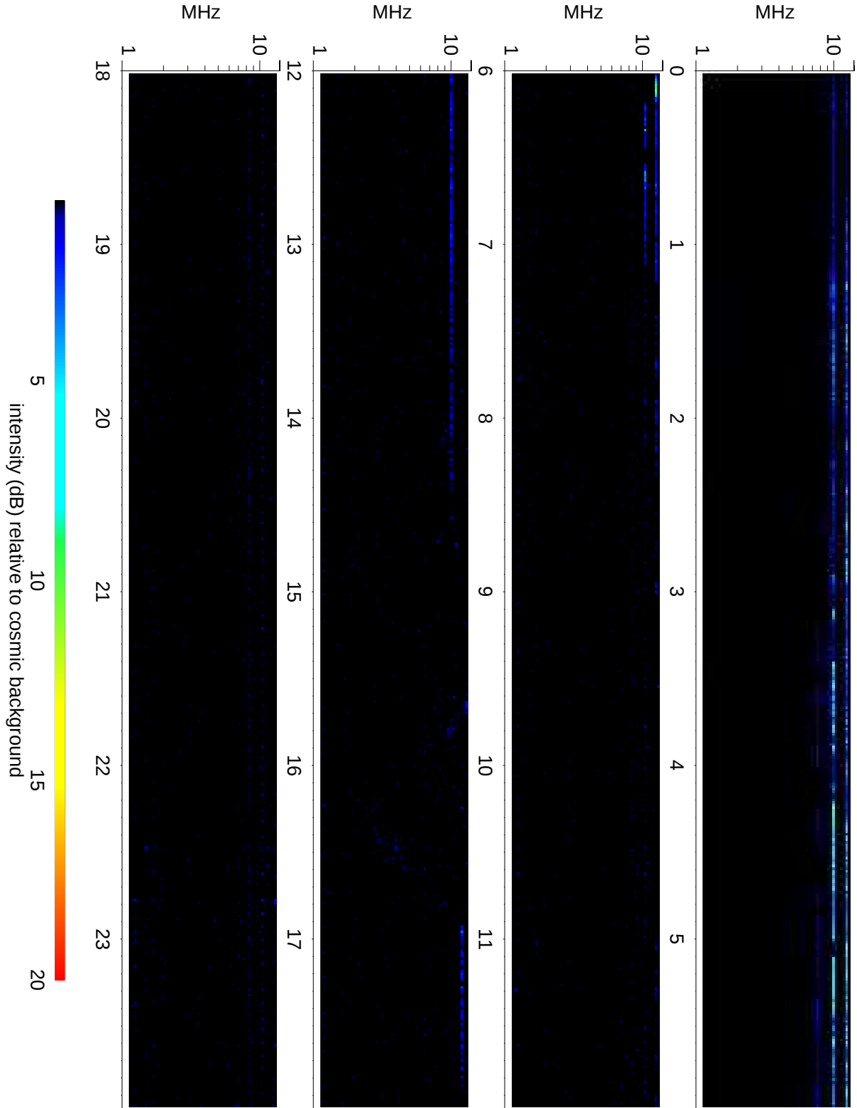
Wind Waves RAD2 receiver: 2019/11/11
