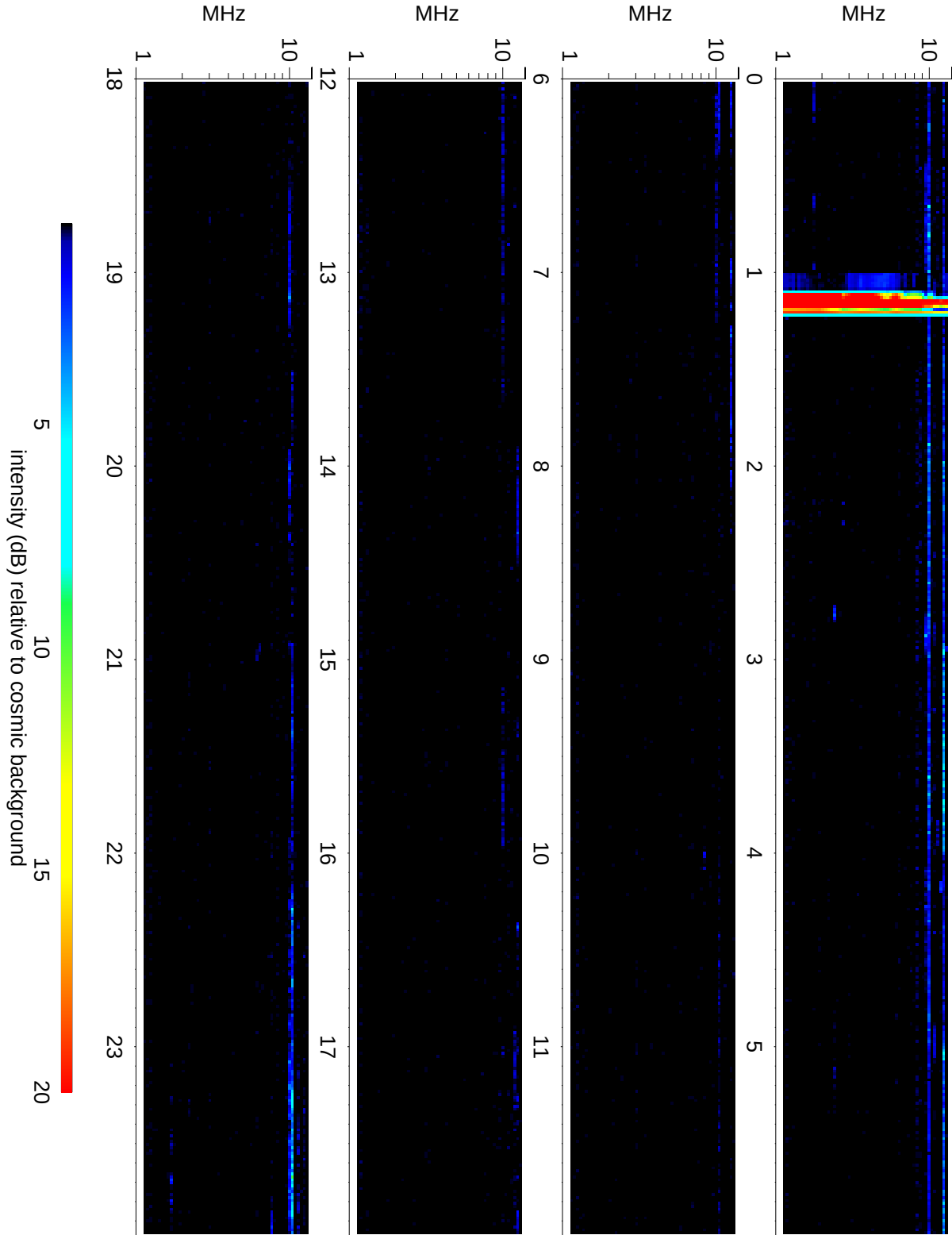
Wind Waves RAD2 receiver: 2019/10/13
