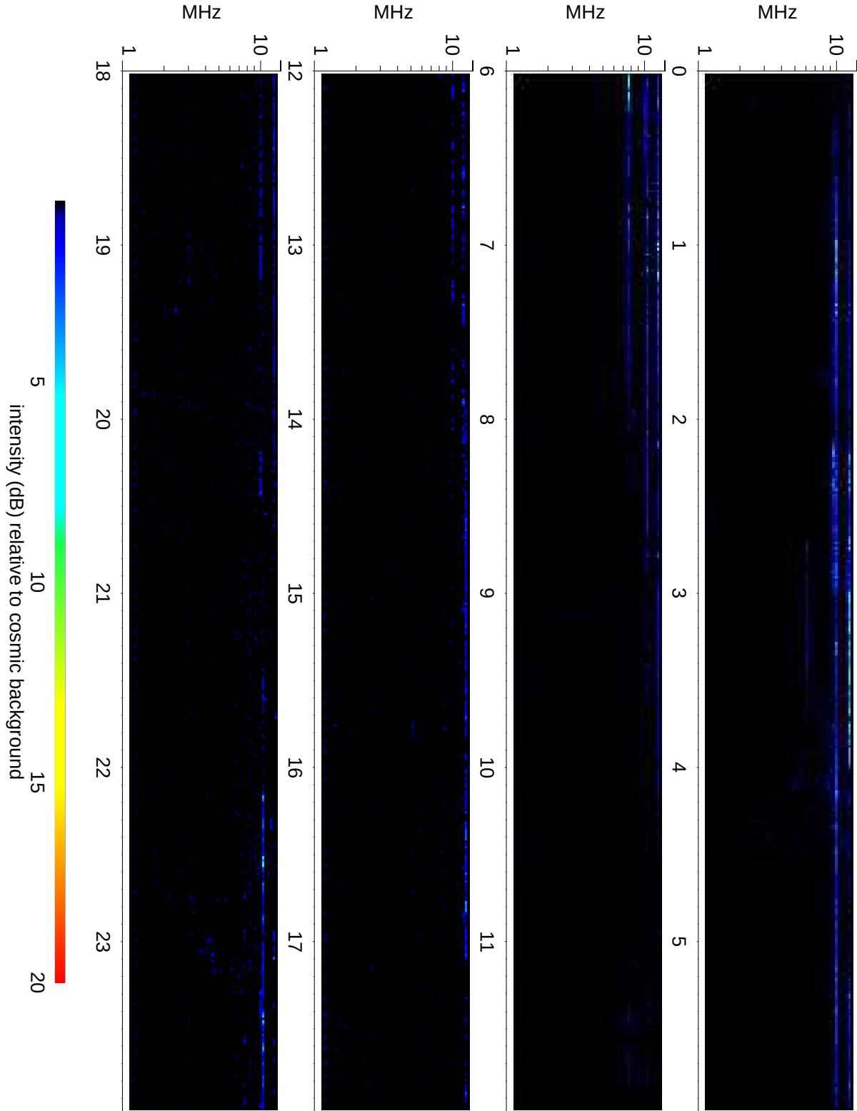
Wind Waves RAD2 receiver: 2019/09/08
