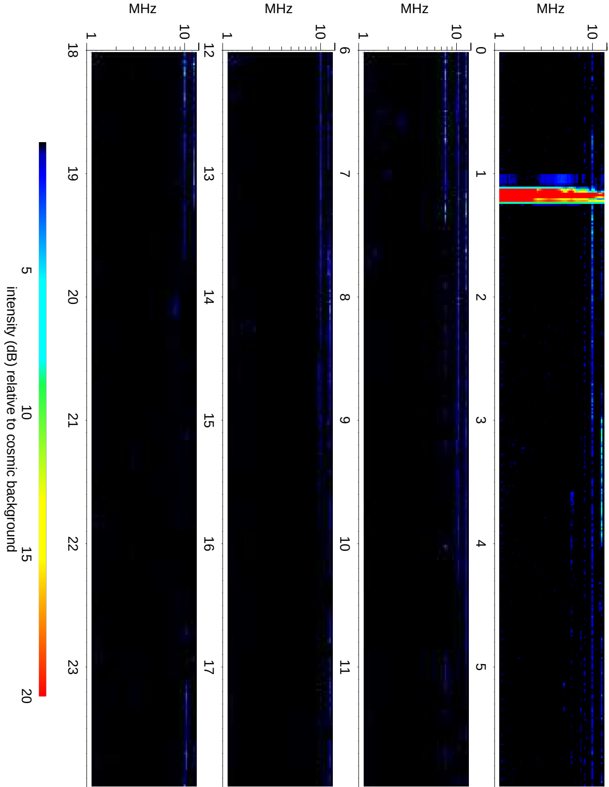
Wind Waves RAD2 receiver: 2019/08/30
