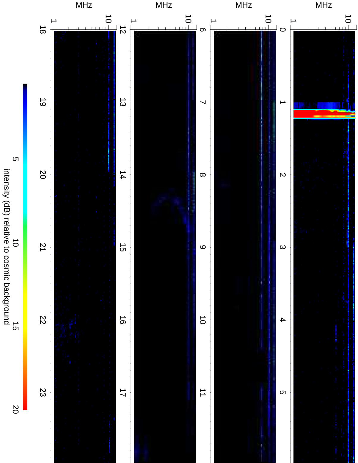
Wind Waves RAD2 receiver: 2019/08/12
