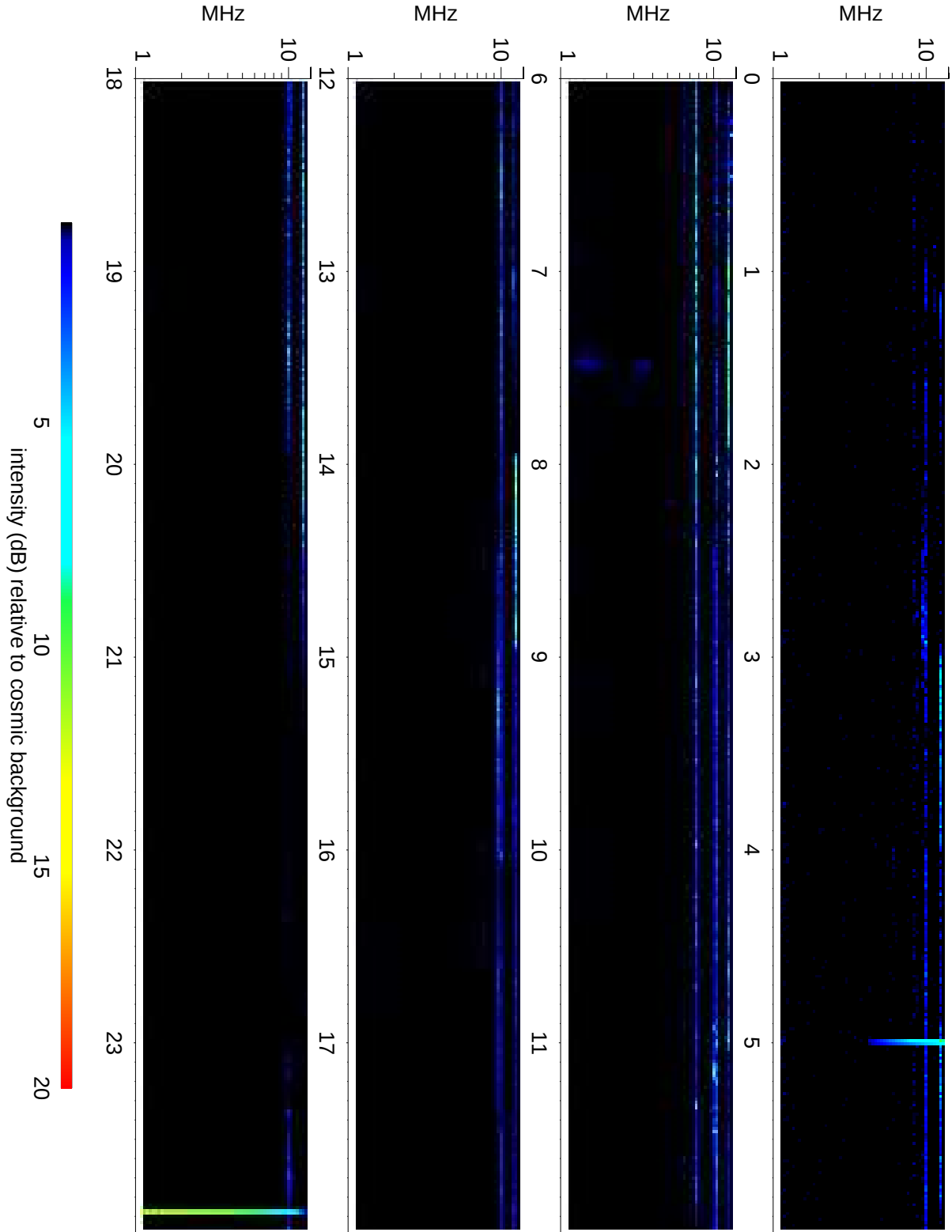
Wind Waves RAD2 receiver: 2019/07/22
