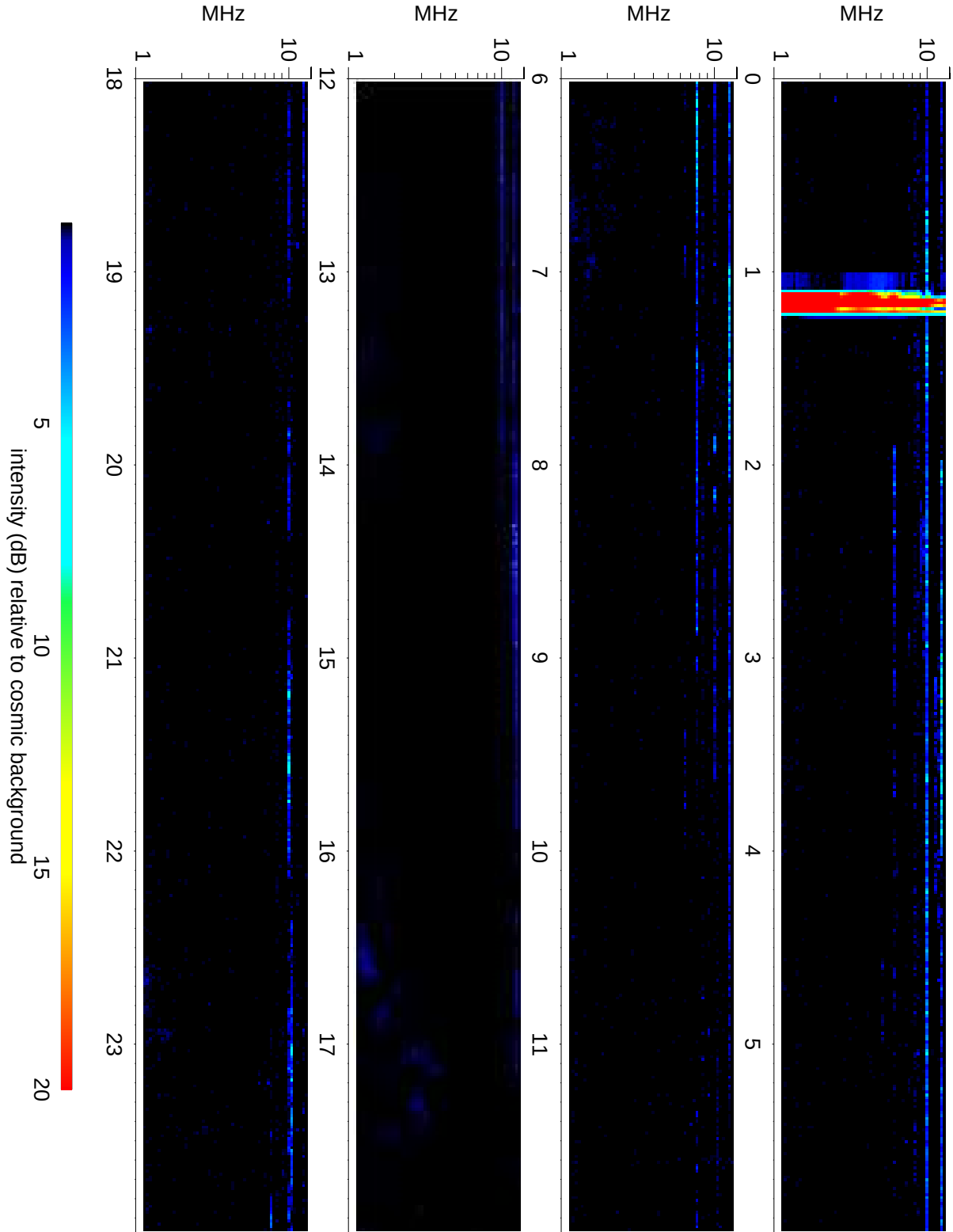
Wind Waves RAD2 receiver: 2019/05/12
