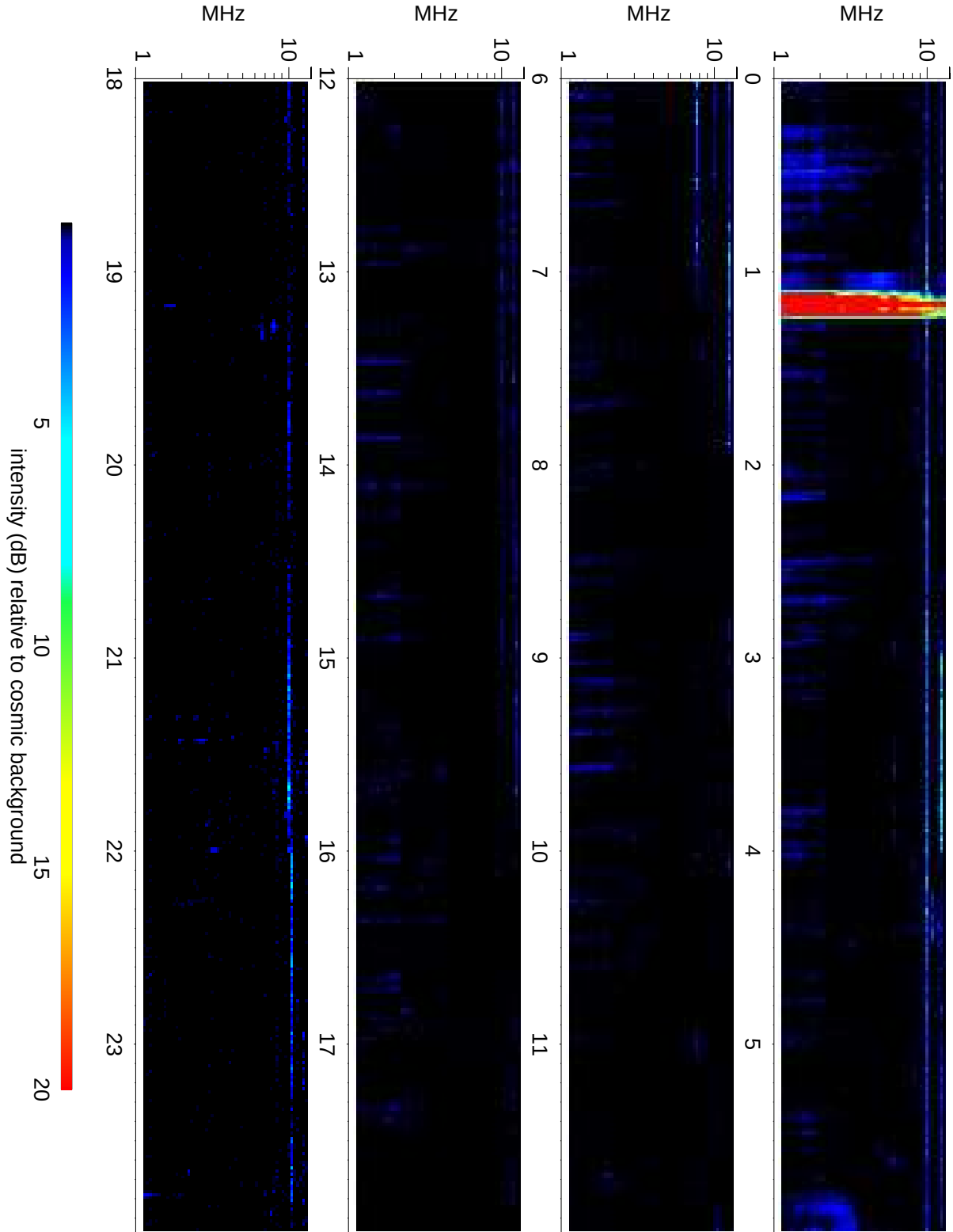
Wind Waves RAD2 receiver: 2019/05/10
