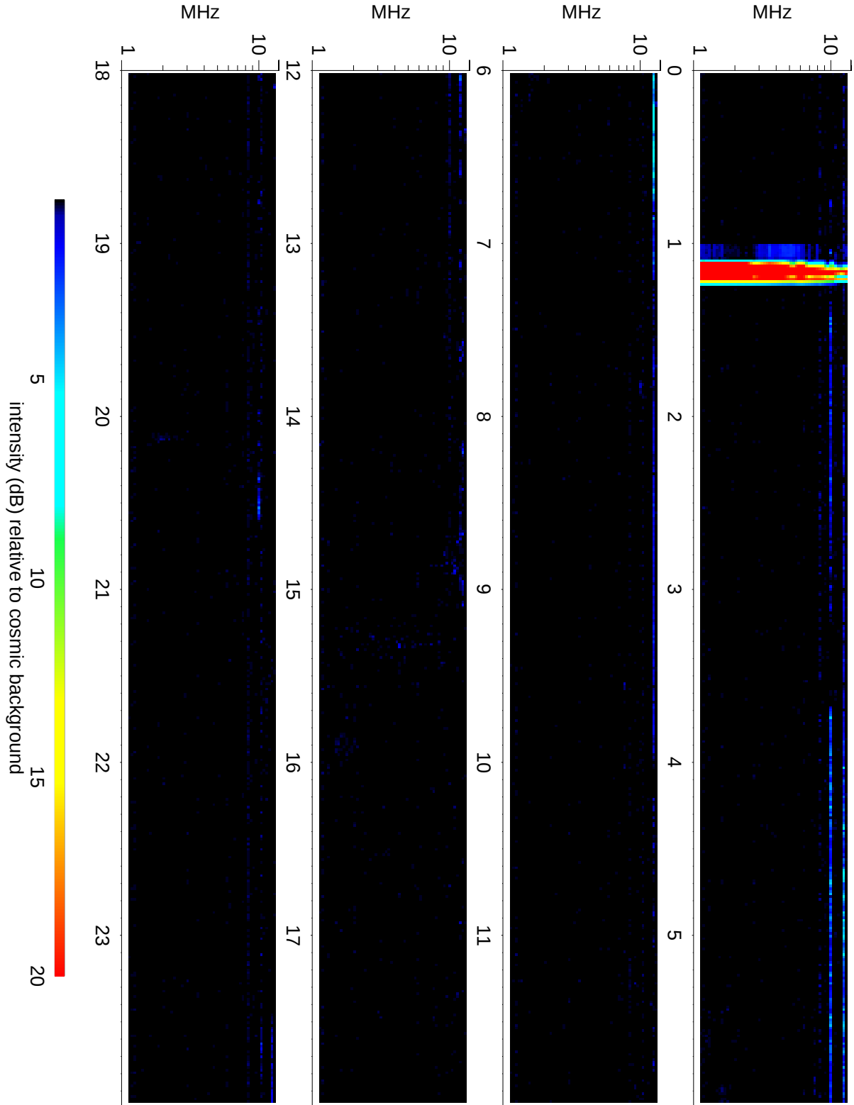
Wind Waves RAD2 receiver: 2019/03/03
