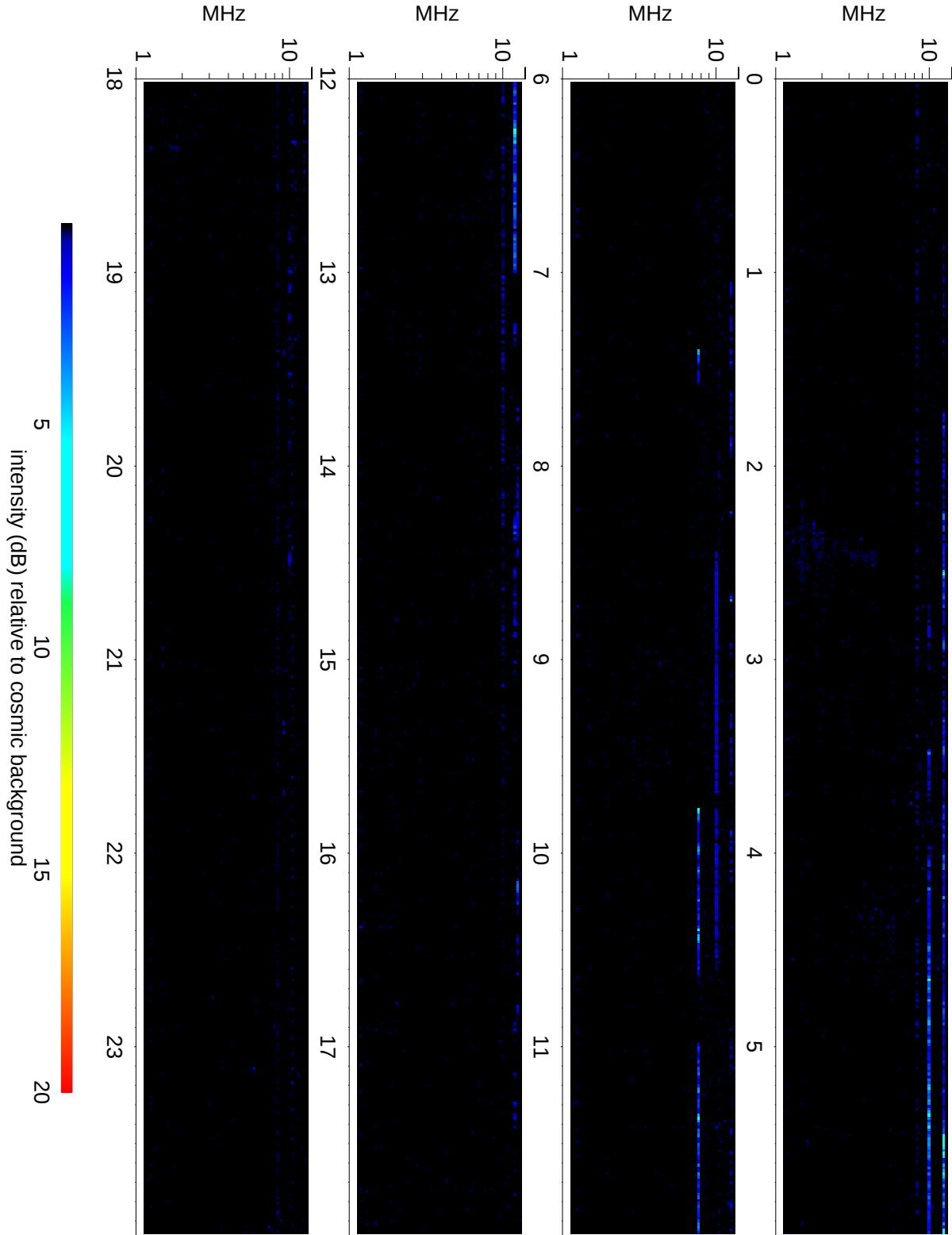
Wind Waves RAD2 receiver: 2019/02/12
