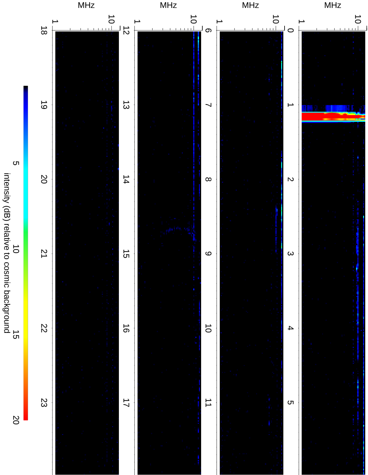
Wind Waves RAD2 receiver: 2019/02/09
