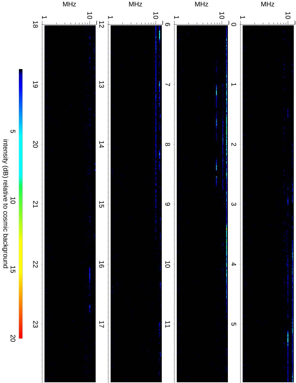
Wind Waves RAD2 receiver: 2019/01/27
