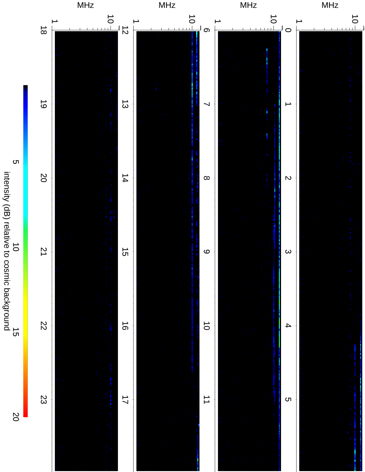
Wind Waves RAD2 receiver: 2019/01/13
