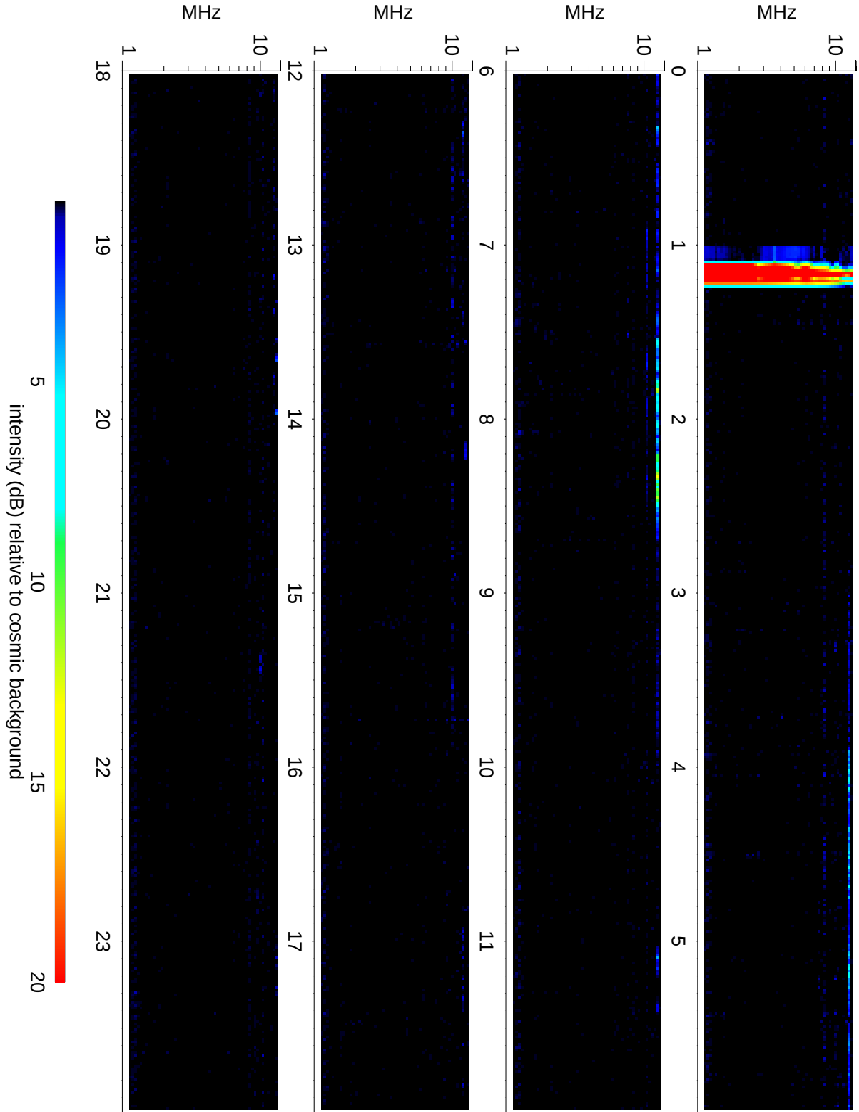
Wind Waves RAD2 receiver: 2018/12/16
