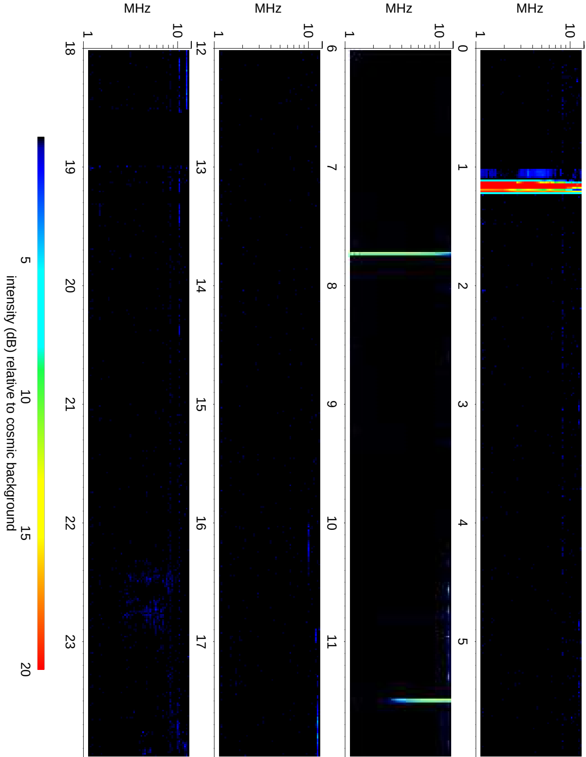
Wind Waves RAD2 receiver: 2015/11/18
