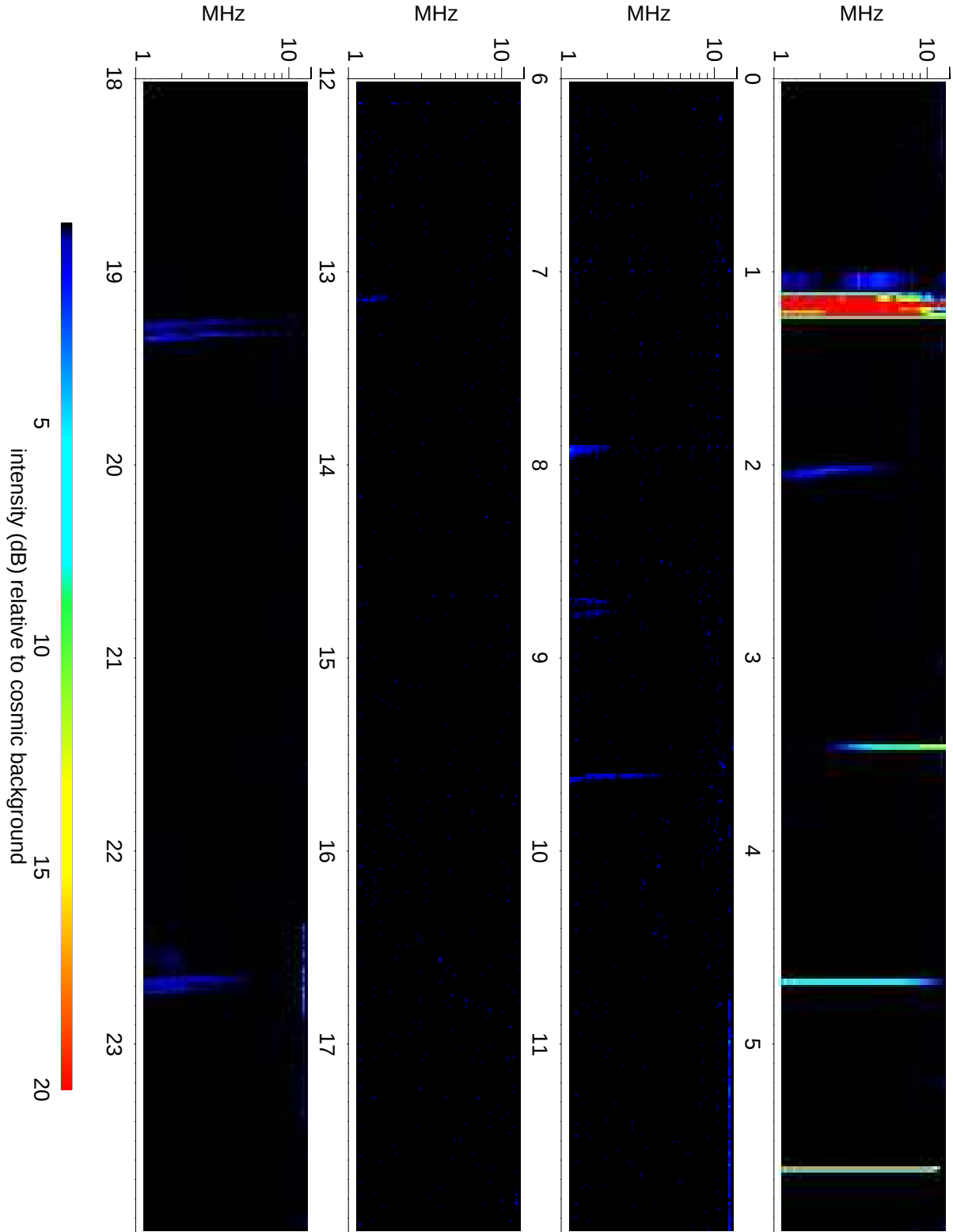
Wind Waves RAD2 receiver: 2015/11/14
