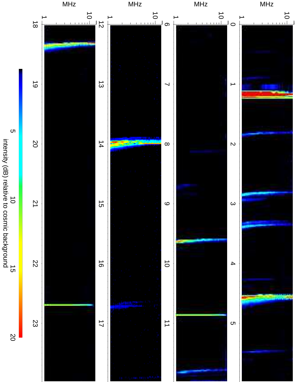
Wind Waves RAD2 receiver: 2015/10/21
