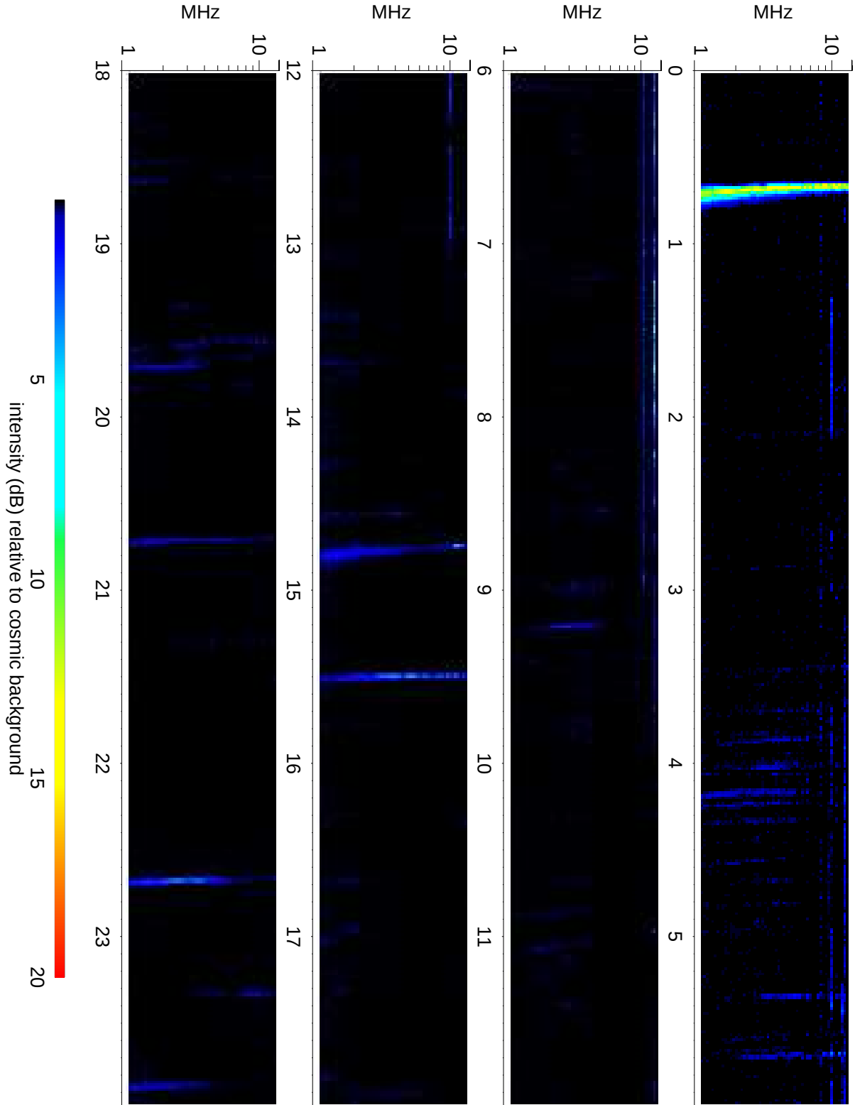
Wind Waves RAD2 receiver: 2015/09/14
