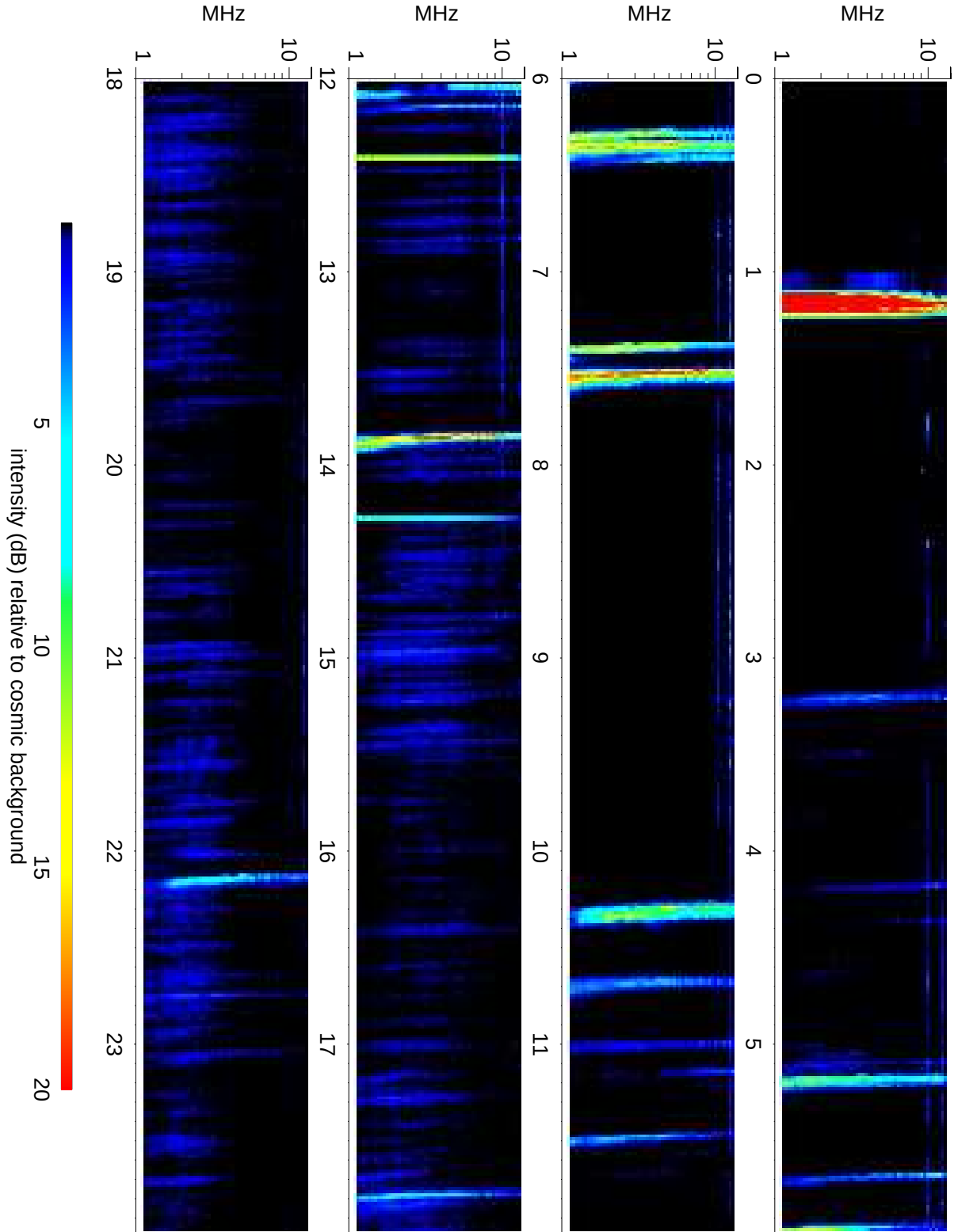
Wind Waves RAD2 receiver: 2015/08/24
