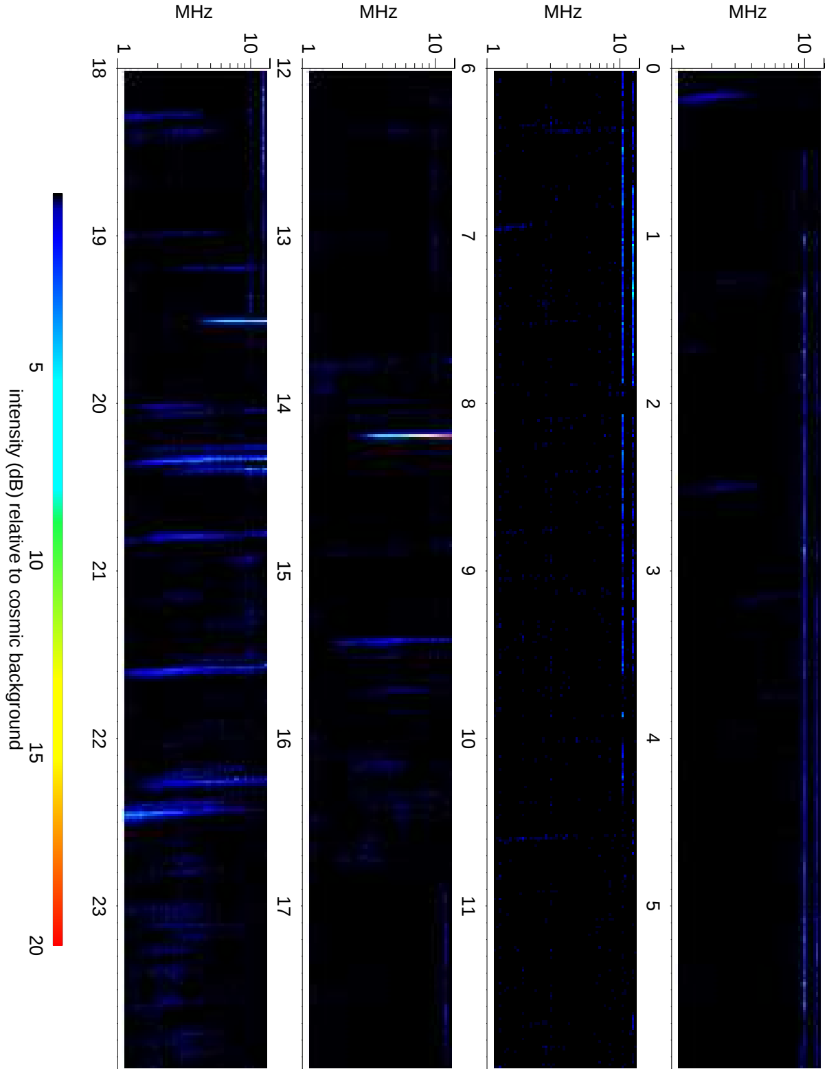
Wind Waves RAD2 receiver: 2015/07/06
