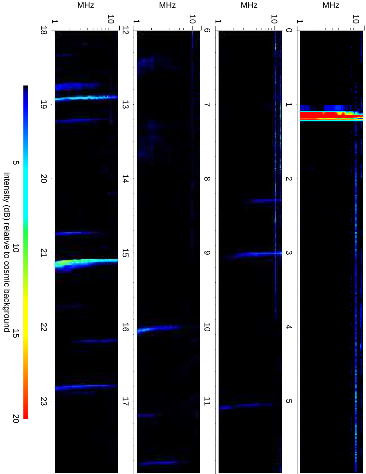
Wind Waves RAD2 receiver: 2015/07/03
