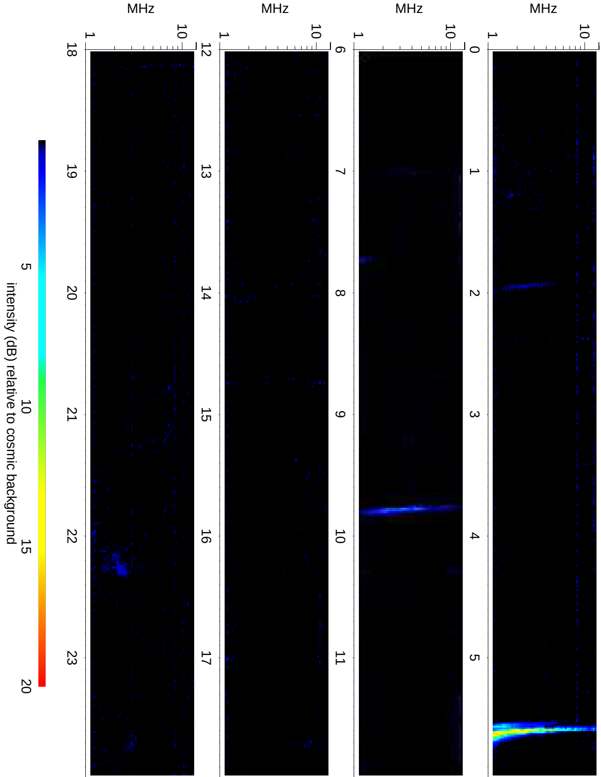
Wind Waves RAD2 receiver: 2015/04/27
