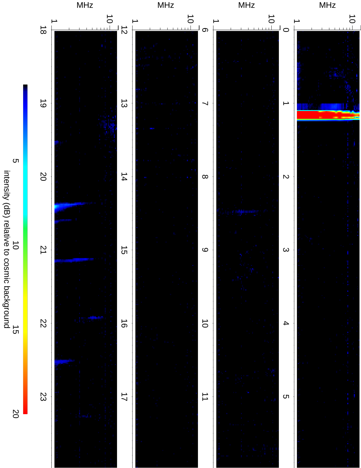
Wind Waves RAD2 receiver: 2015/04/24
