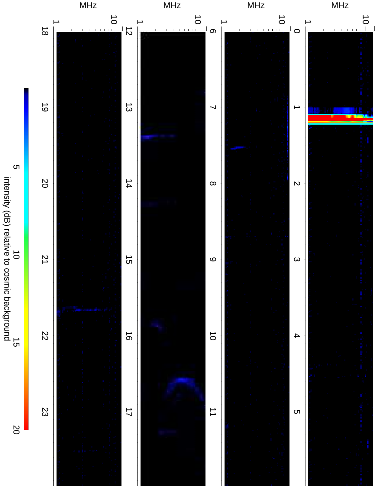
Wind Waves RAD2 receiver: 2015/04/18
