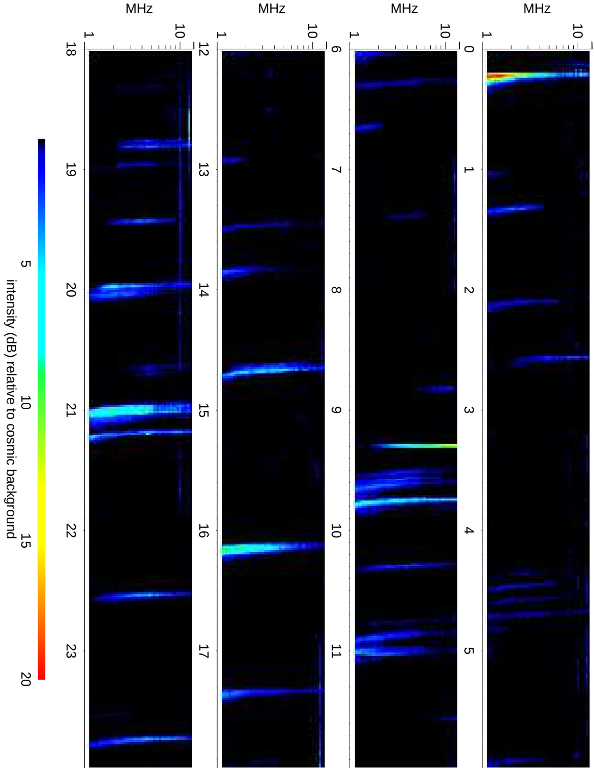
Wind Waves RAD2 receiver: 2015/04/11
