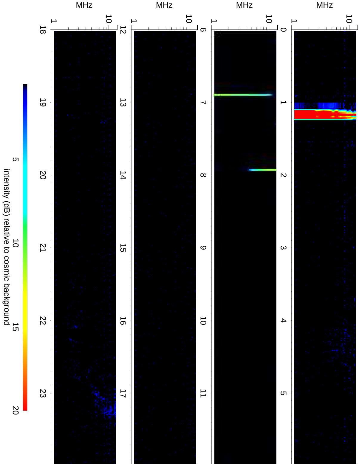
Wind Waves RAD2 receiver: 2015/03/23
