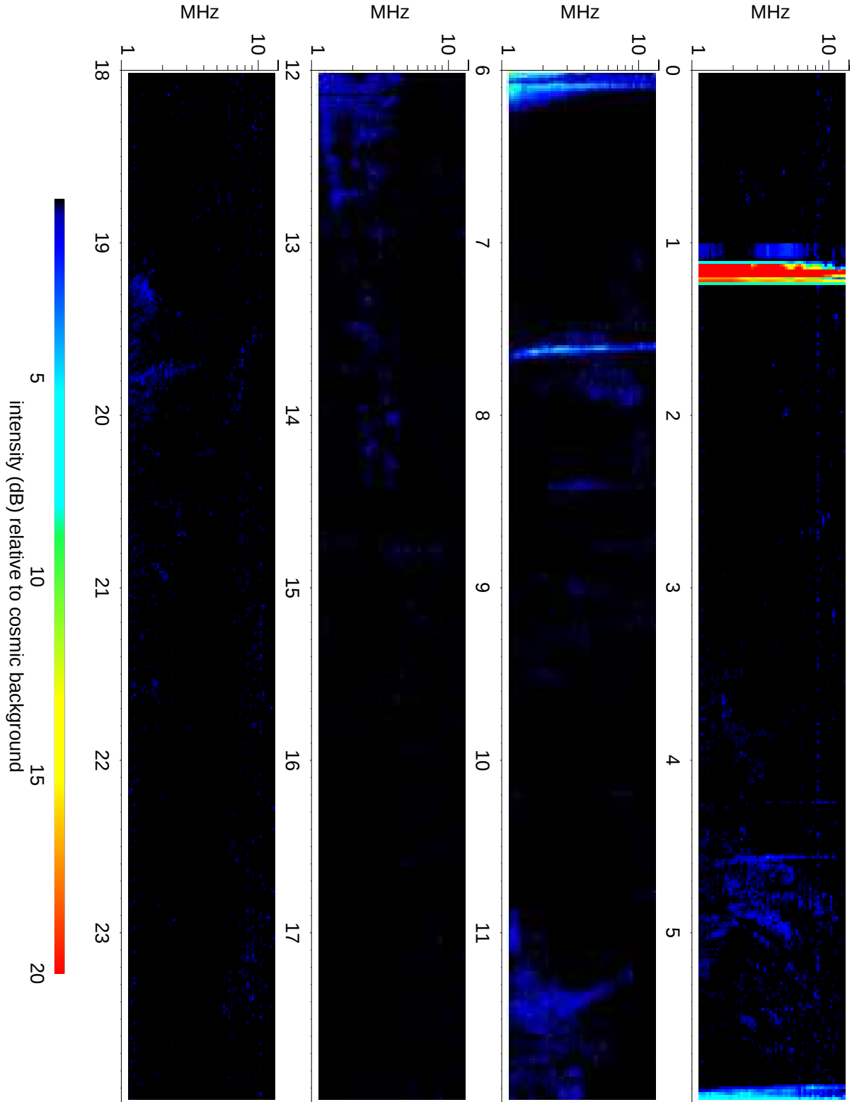
Wind Waves RAD2 receiver: 2015/03/13
