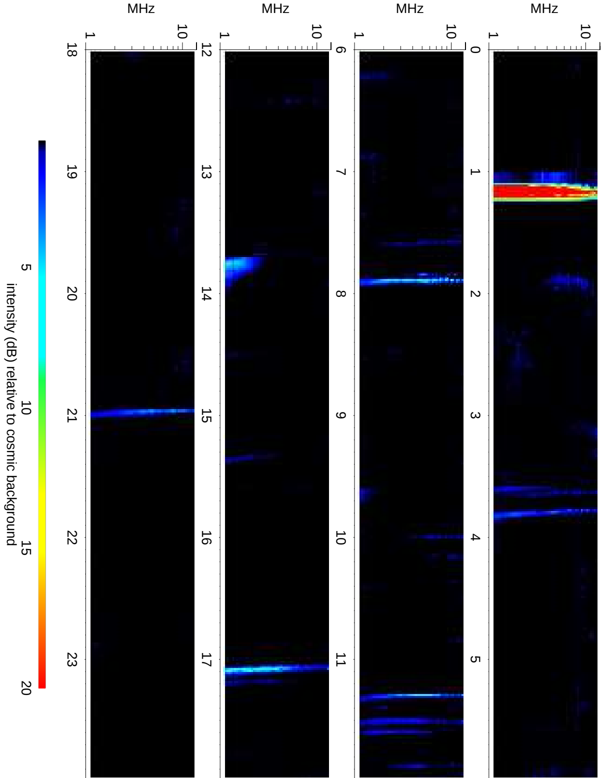
Wind Waves RAD2 receiver: 2015/02/21
