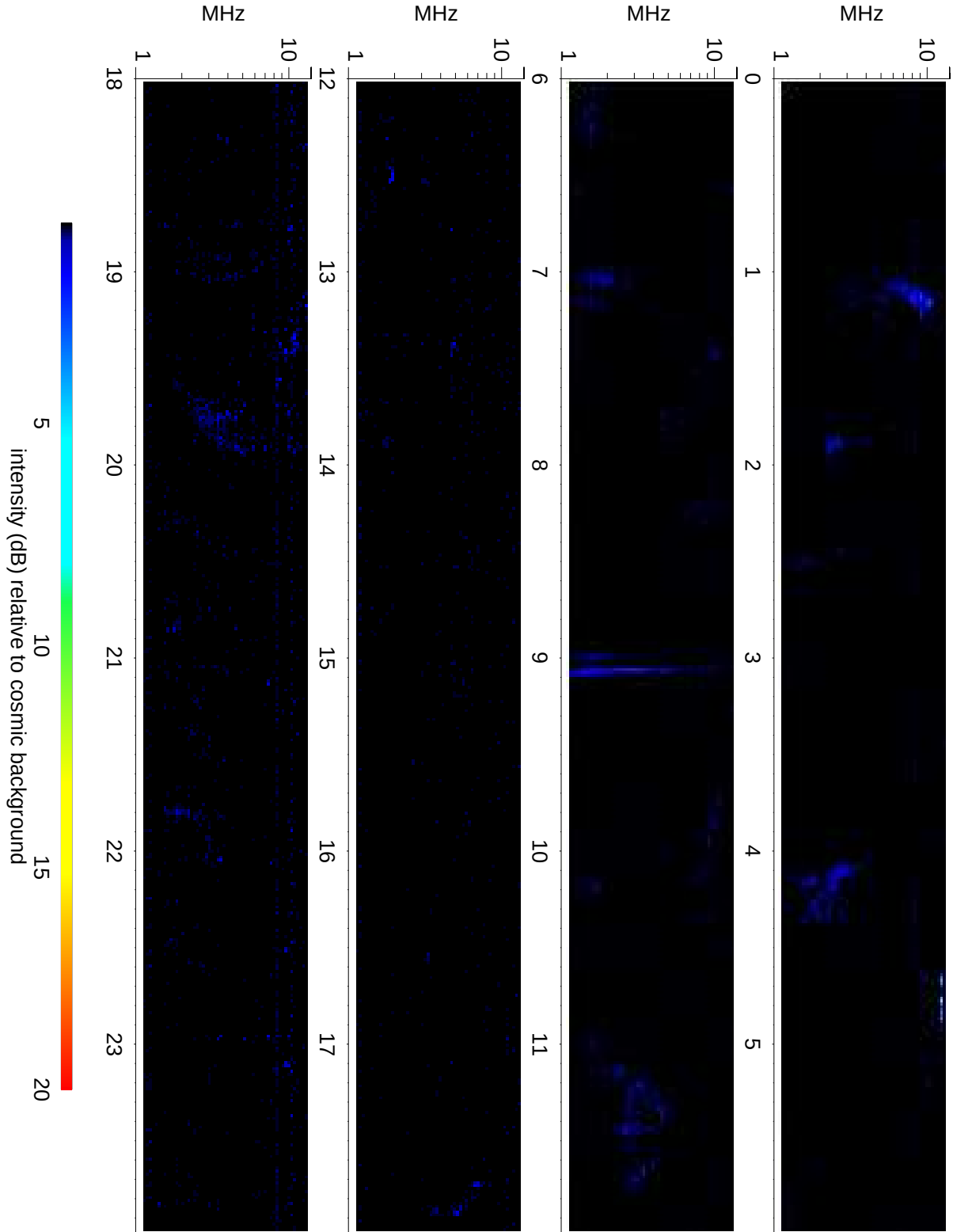
Wind Waves RAD2 receiver: 2015/02/14
