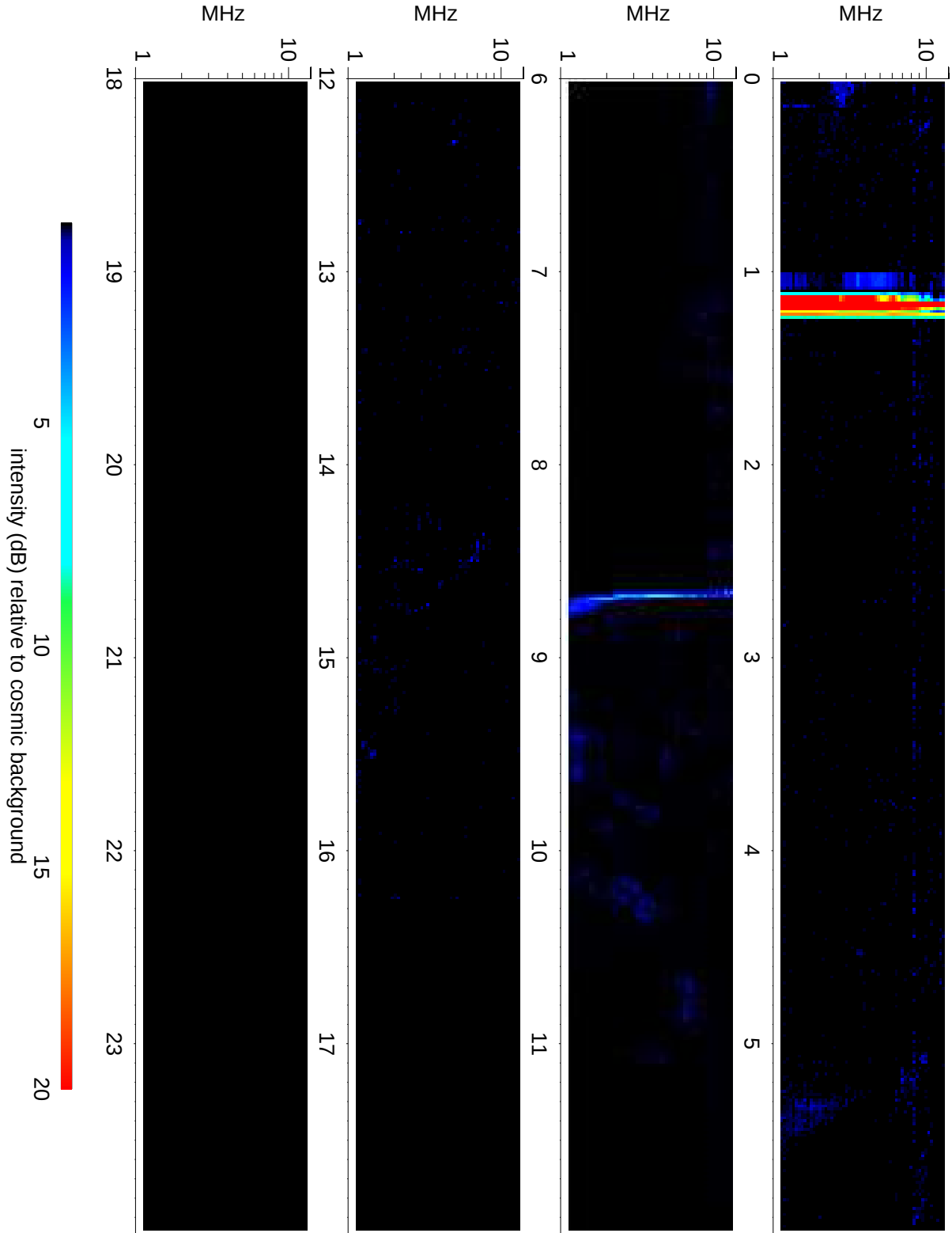
Wind Waves RAD2 receiver: 2015/02/11
