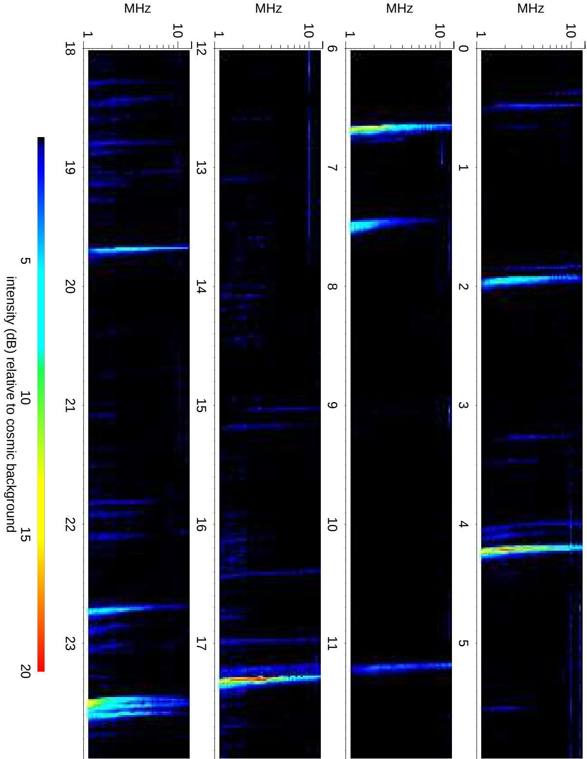
Wind Waves RAD2 receiver: 2014/08/19
