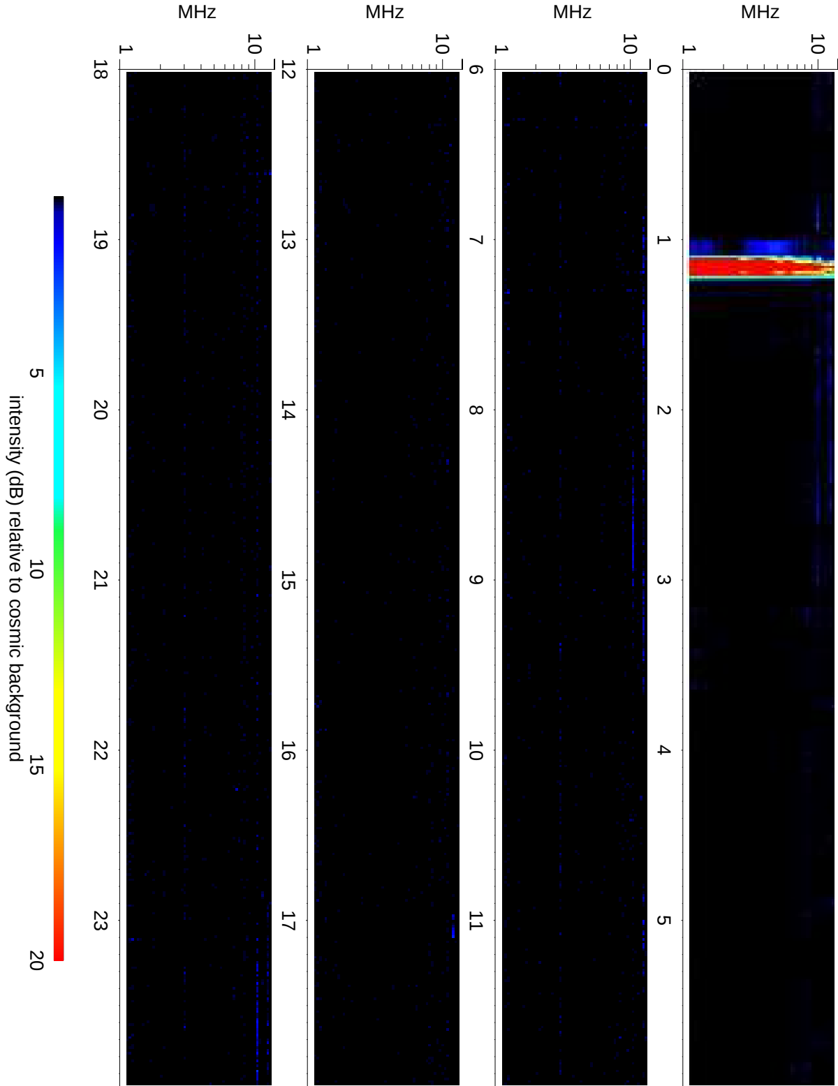
Wind Waves RAD2 receiver: 2014/05/22
