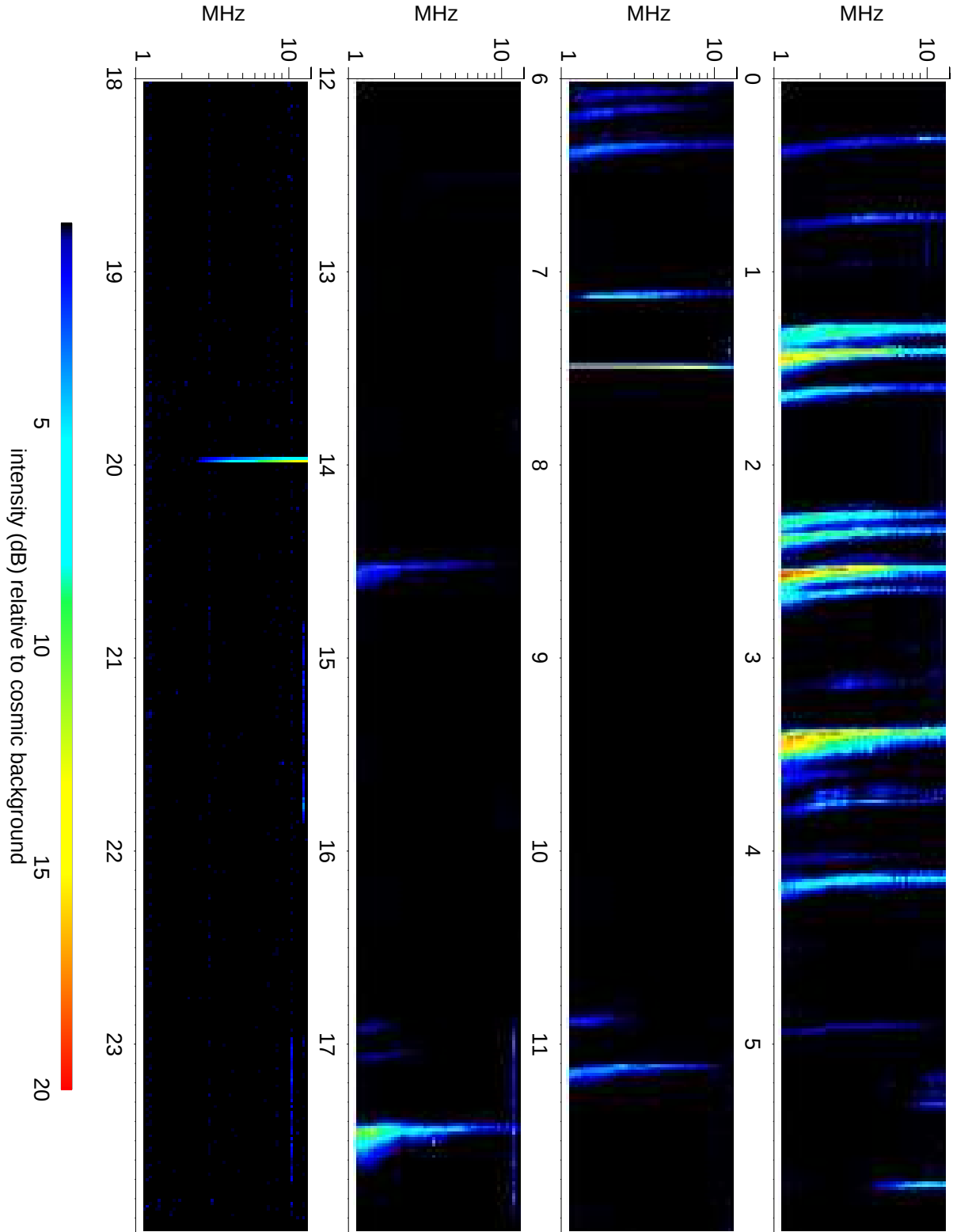
Wind Waves RAD2 receiver: 2014/05/01
