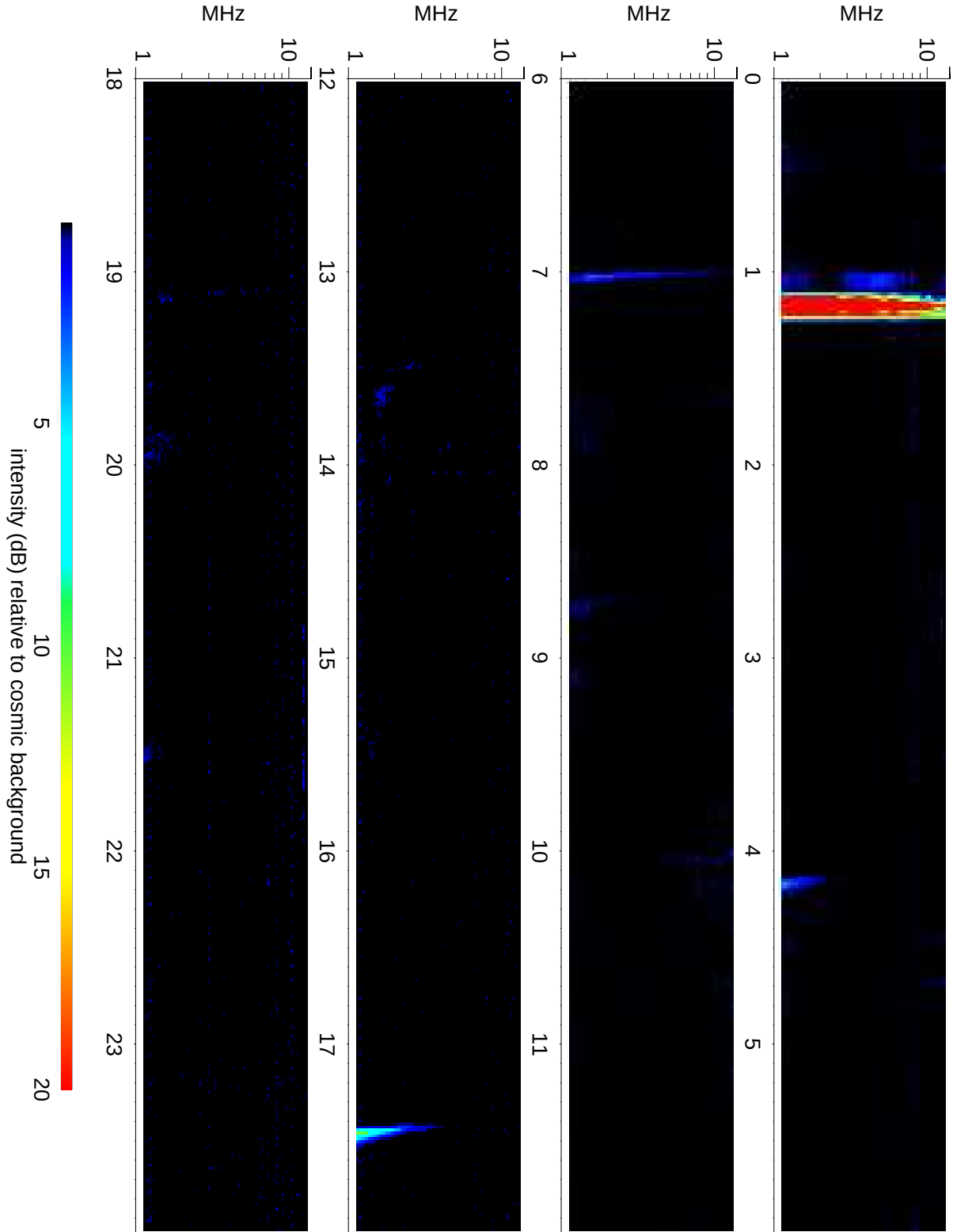
Wind Waves RAD2 receiver: 2014/04/24
