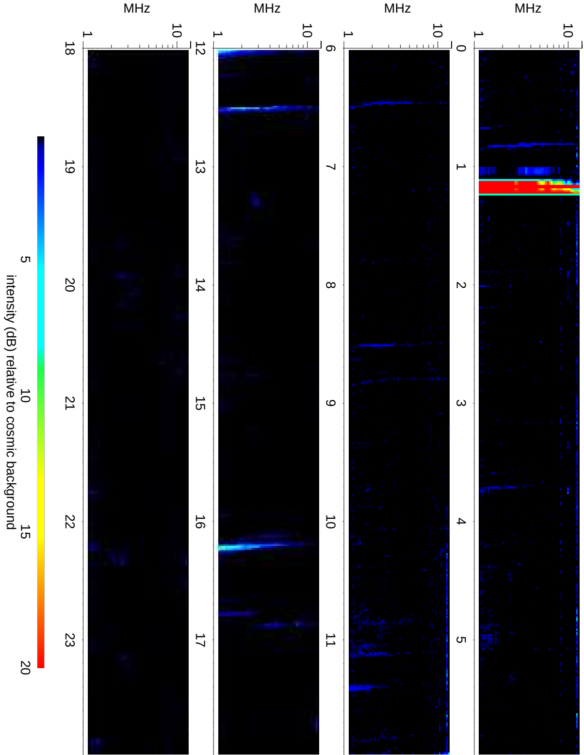
Wind Waves RAD2 receiver: 2012/11/29
