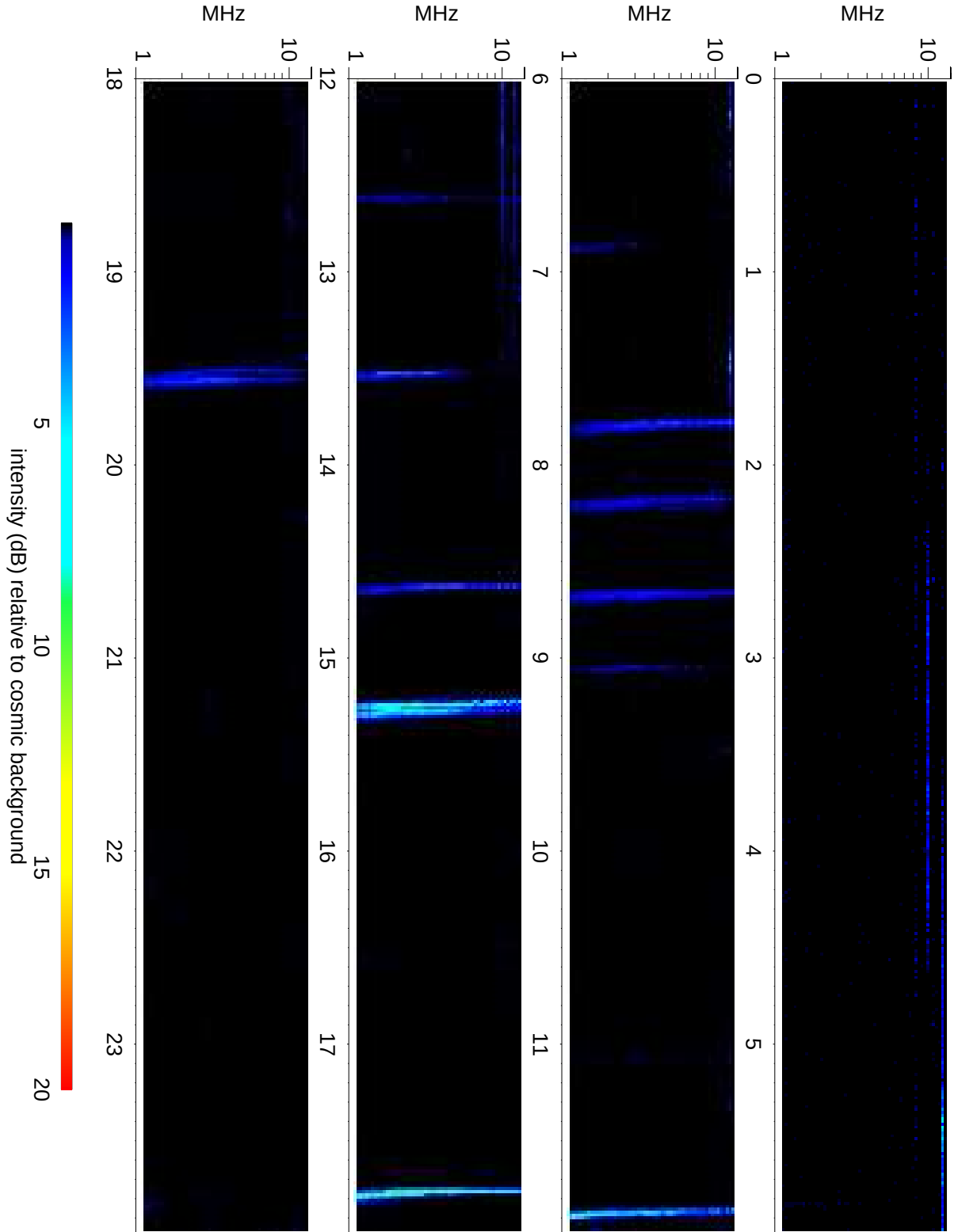
Wind Waves RAD2 receiver: 2012/08/22
