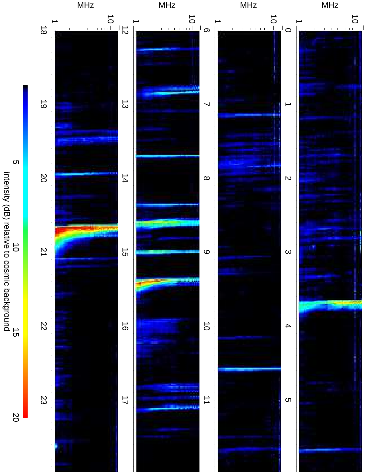
Wind Waves RAD2 receiver: 2012/07/03
