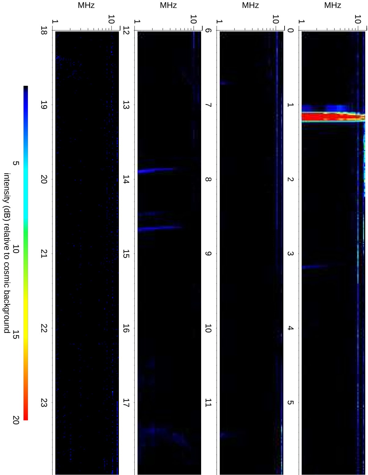
Wind Waves RAD2 receiver: 2012/06/24
