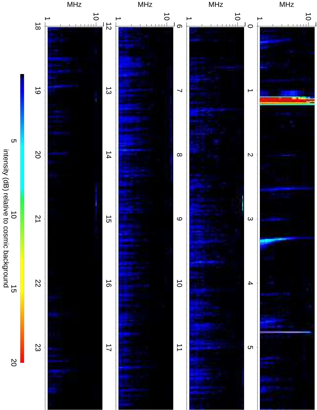
Wind Waves RAD2 receiver: 2012/03/18
