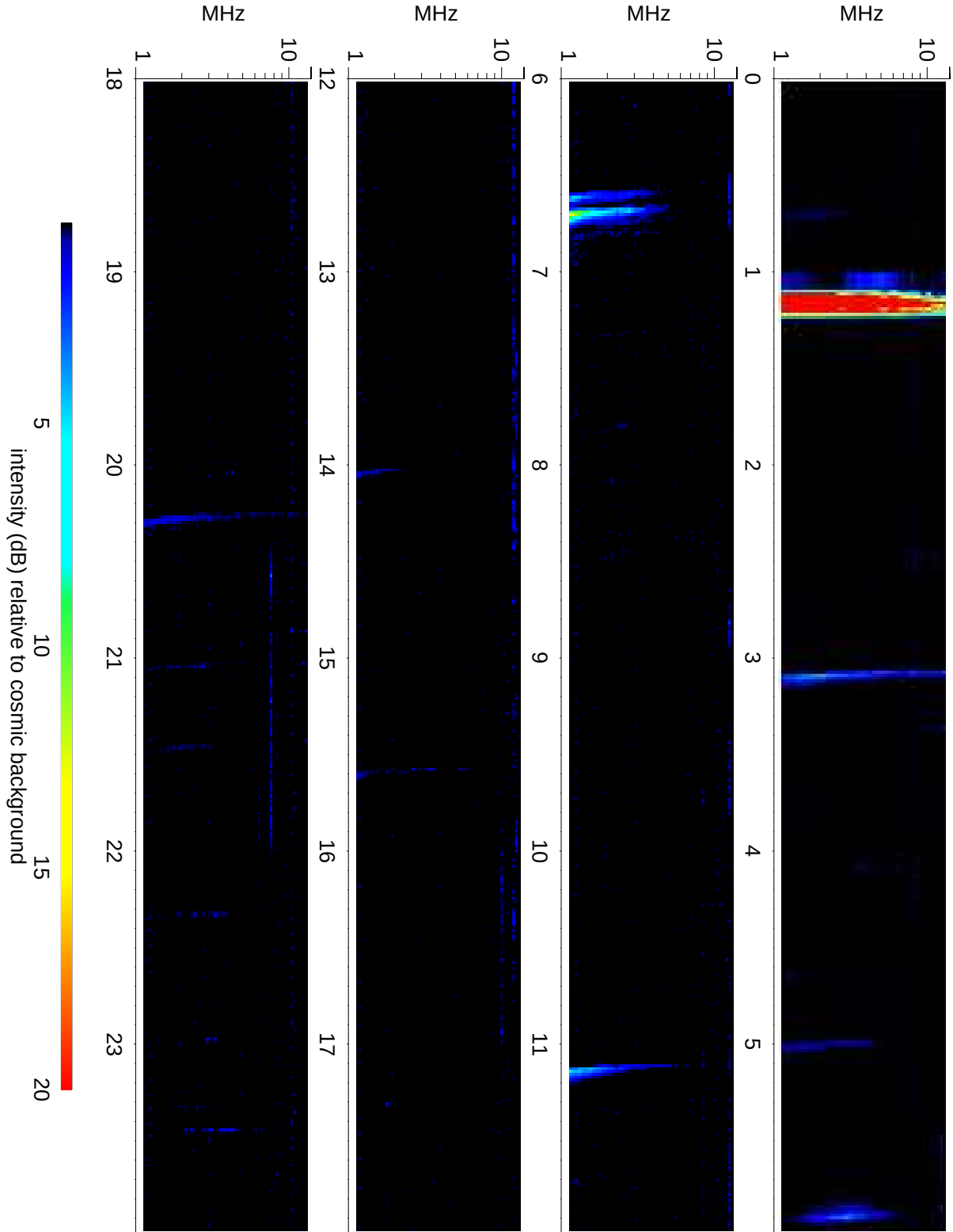
Wind Waves RAD2 receiver: 2012/03/16
