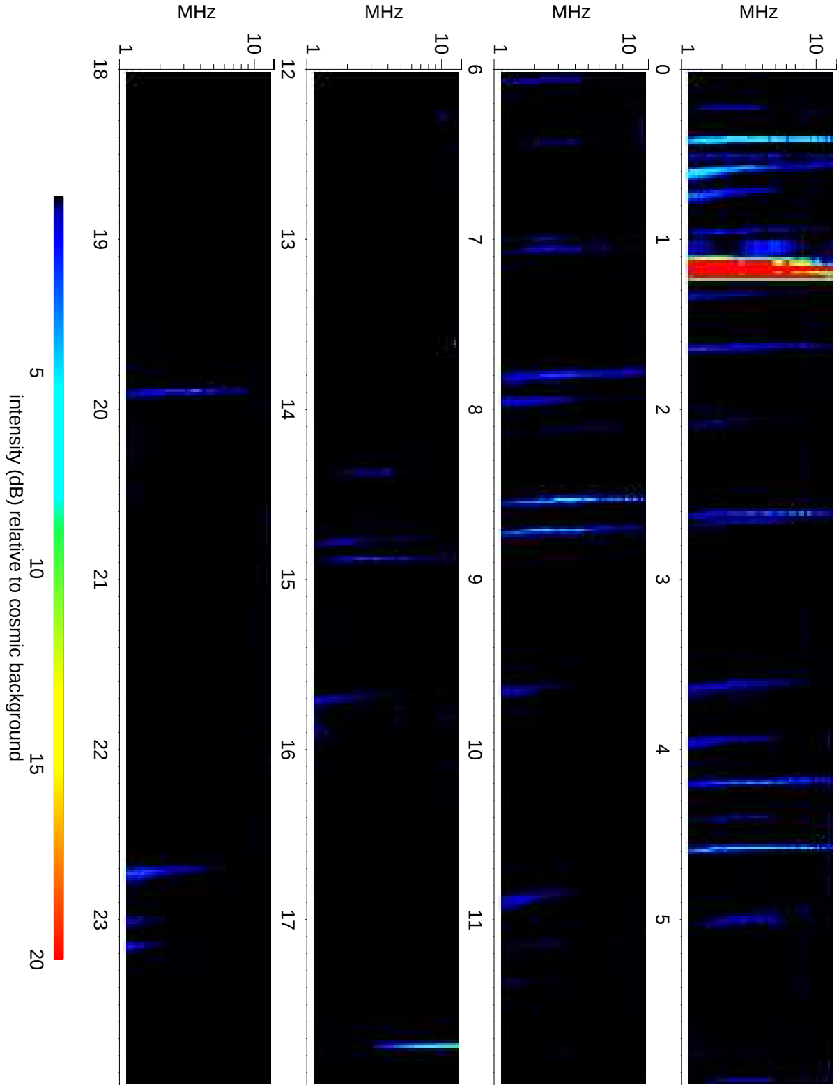
Wind Waves RAD2 receiver: 2012/03/14
