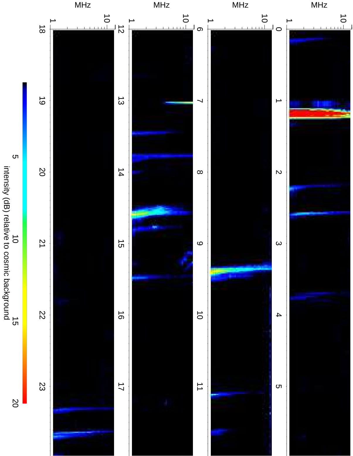
Wind Waves RAD2 receiver: 2012/01/02
