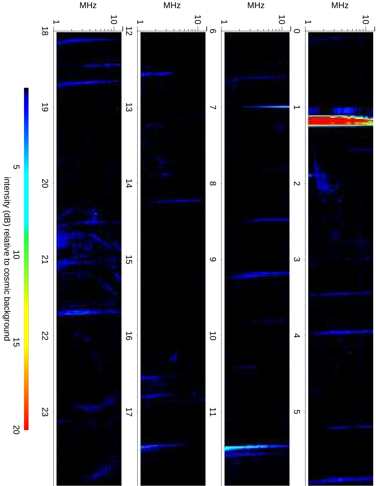
Wind Waves RAD2 receiver: 2011/11/02
