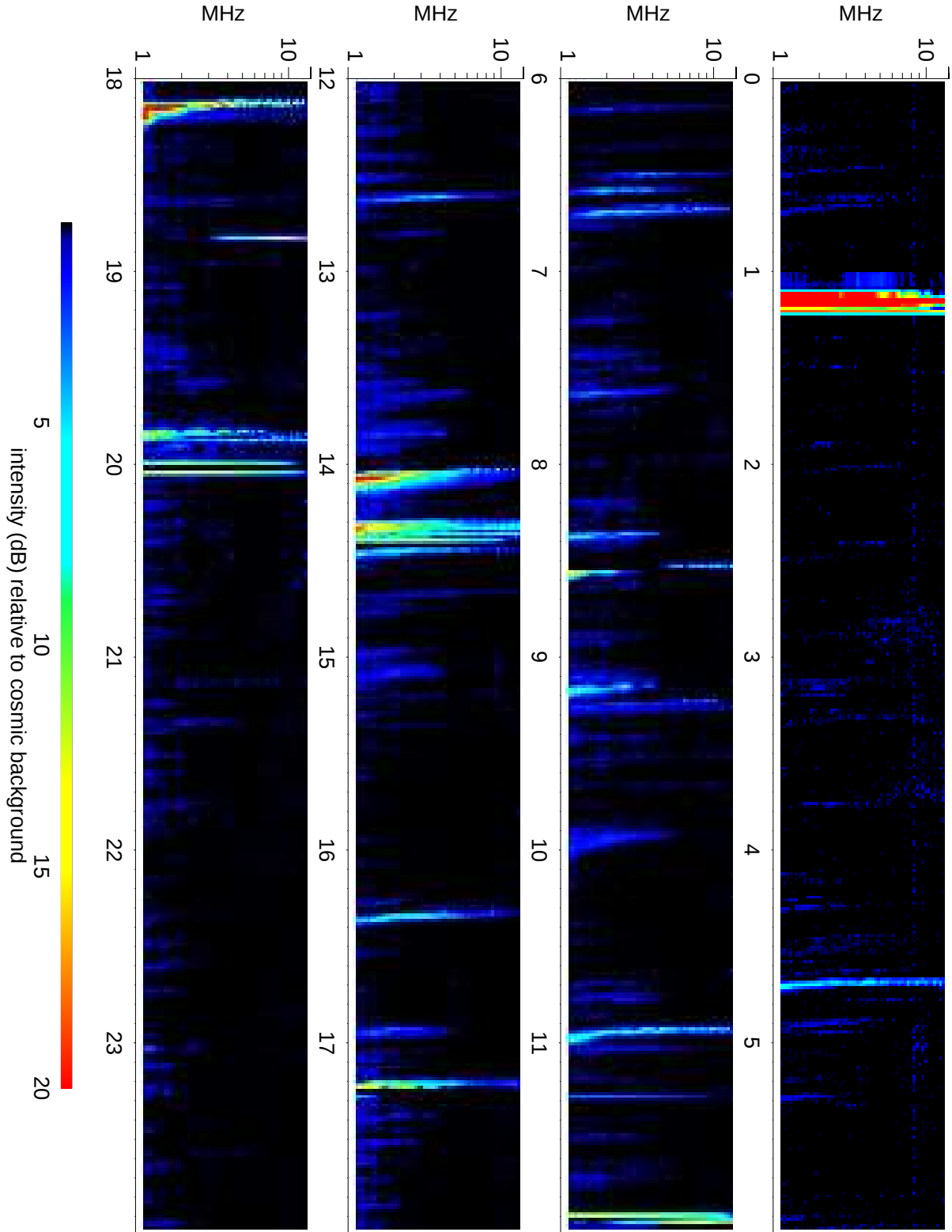
Wind Waves RAD2 receiver: 2011/10/17
