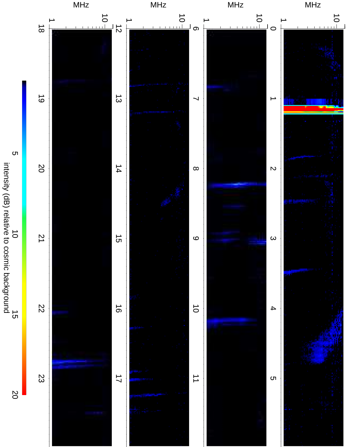
Wind Waves RAD2 receiver: 2011/10/09
