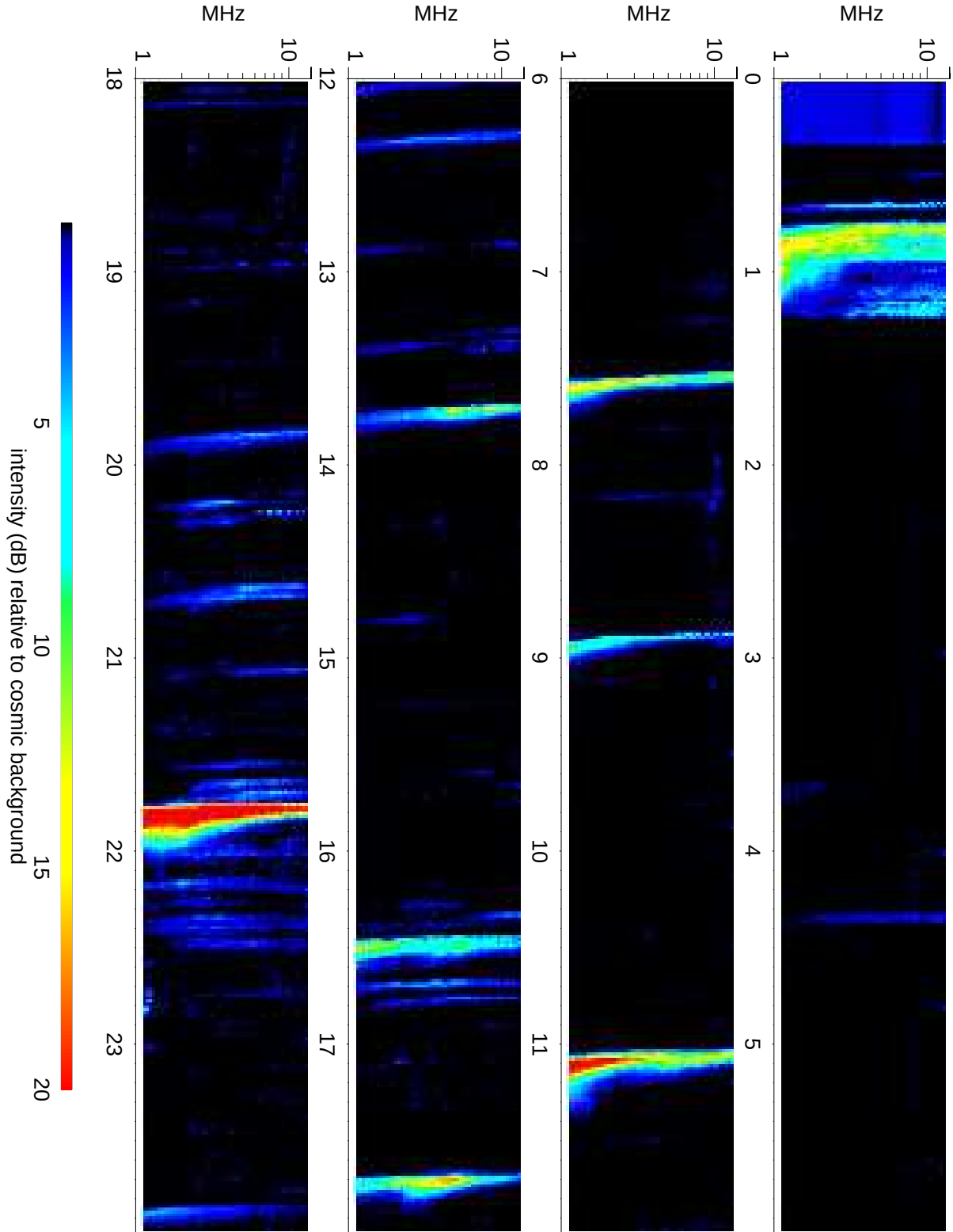
Wind Waves RAD2 receiver: 2011/10/02
