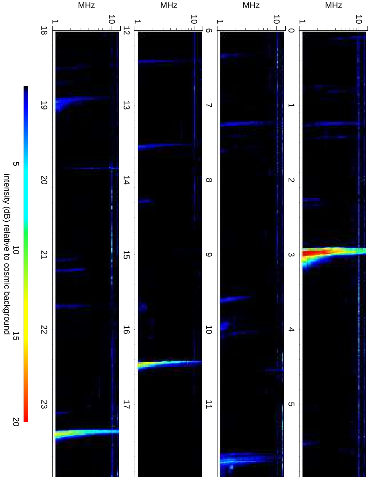
Wind Waves RAD2 receiver: 2011/07/08
