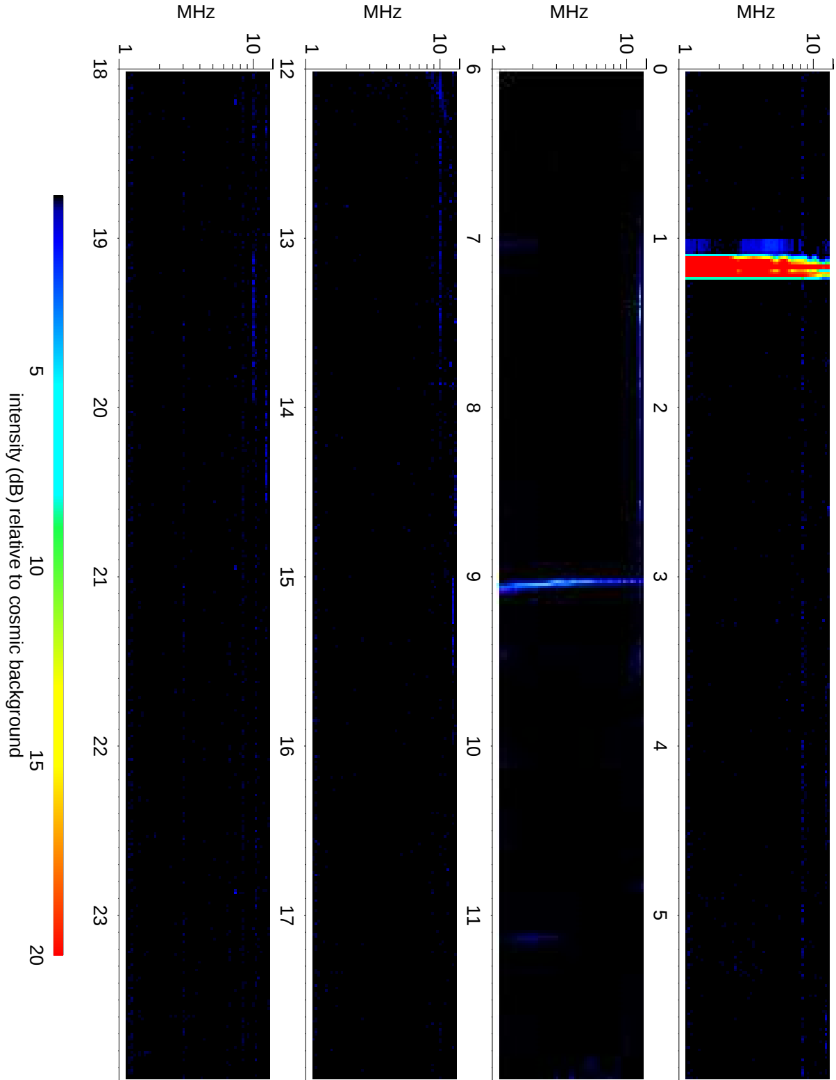
Wind Waves RAD2 receiver: 2011/04/28
