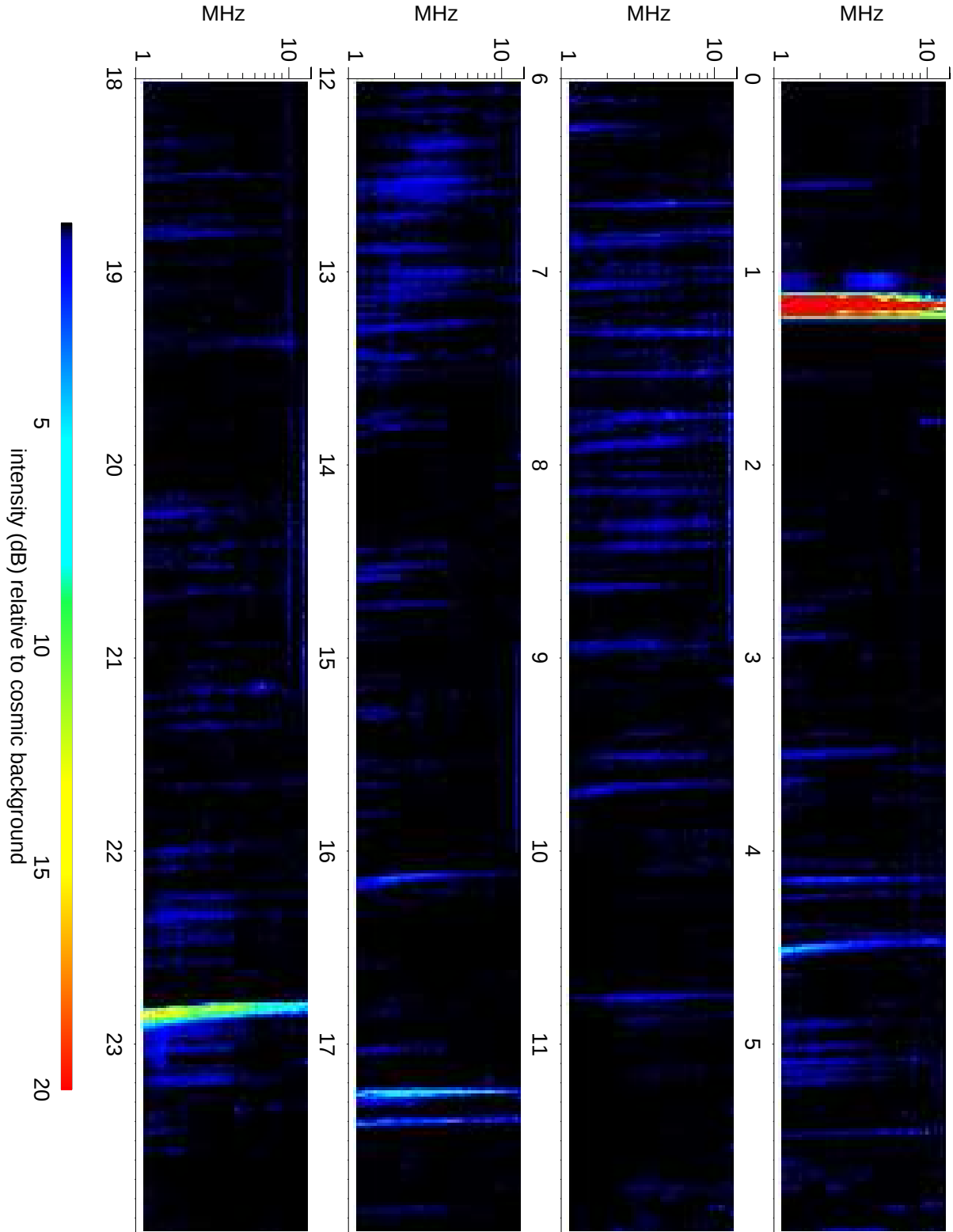
Wind Waves RAD2 receiver: 2011/04/02
