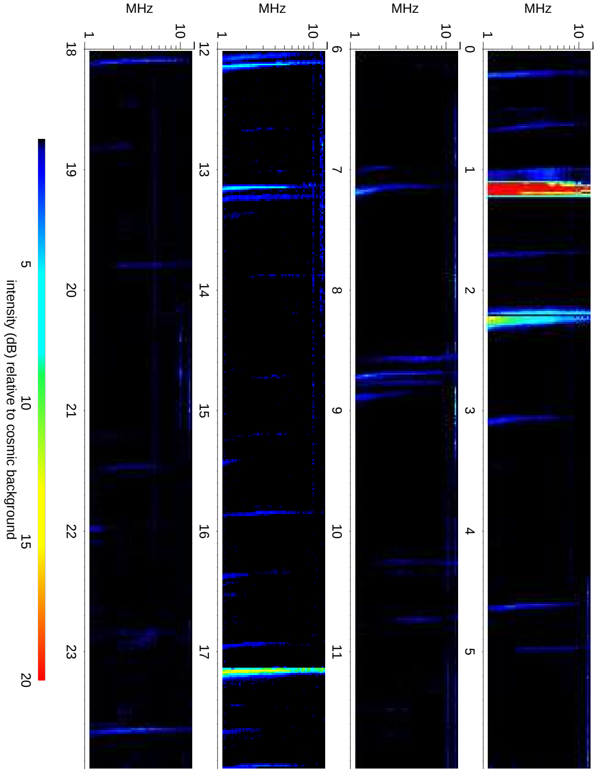
Wind Waves RAD2 receiver: 2011/03/23
